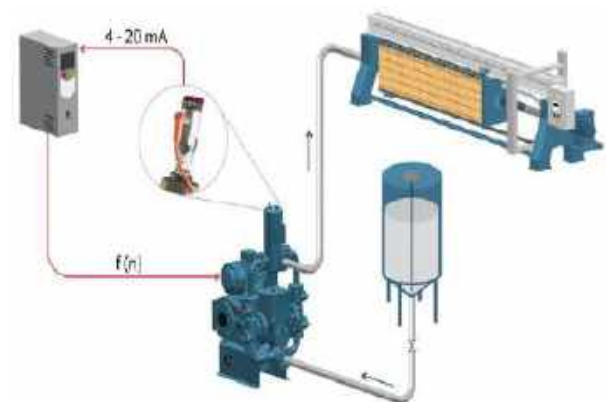
ABEL HM, comprehensive and integrated solution for filter press
