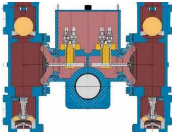
ABEL HM cone valve and ball valve design
