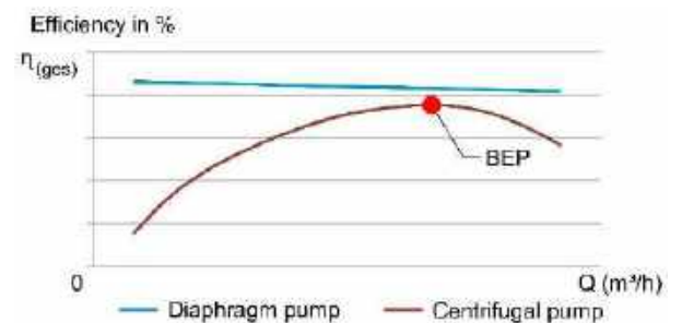
Efficiency vs. operating flow
