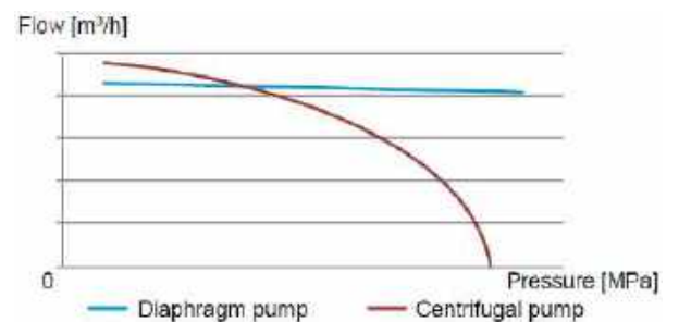
Flow vs. pressure operating curve
